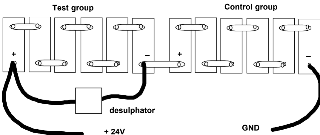
Fig 5 Test arrangement for the trial. For 24 V systems both sides are identical with the battery string being divided into two equal parts.. For 48V systems, the control component would consist of the balance of the battery bank, equating to 18 cells.
