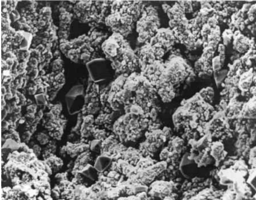
Fig 3 This battery positive plate, magnified 554 times, has been in operation on an emergency vehicle equipped with a de-sulphation device for 11 months. Note the presence of a few large crystals, but otherwise the appearance is similar to the new plate. The battery was performing well, but was removed and torn down so as to carry out this electron microscope inspection.
