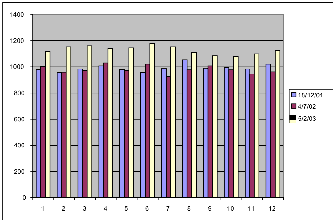
Fig 16 A well maintained set of Century-Yuasa SSR700 tubular plate batteries. The evident improvement in the conductance of the cells at 5/02/03 is largely due to improved charging and equalisation by the householder. However, the TEST group showed an improvement over the CONTROL (-17.5%, -10.38%), indicating that the de-sulphator was quite effective in this instance. This installation, although only having 900 peak watts of PV, had good insolation and low loads.
