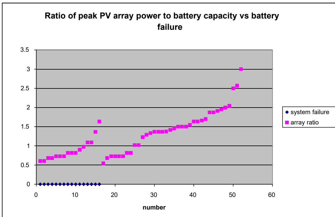
Fig 18 Ratio between the installed peak PV array power (in watts) to incidence of battery failure.
