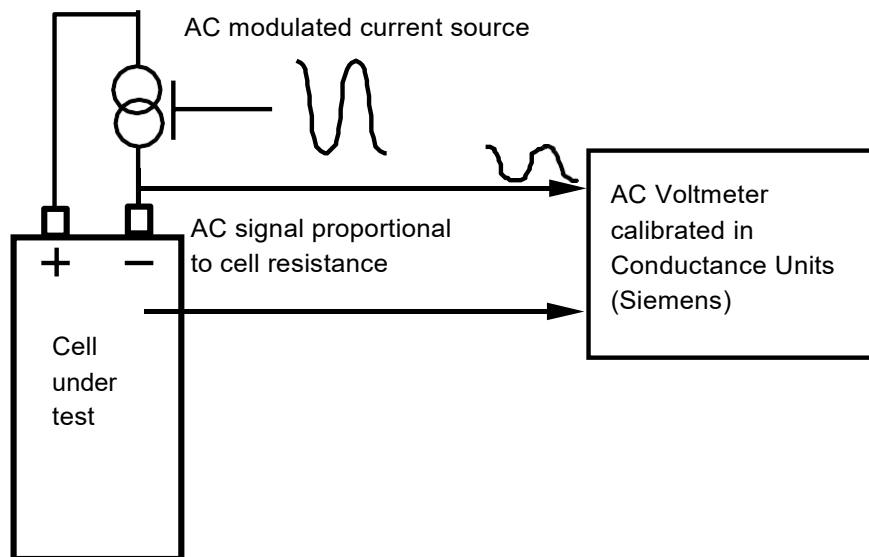
Fig 7 Simplified arrangement for measuring AC conductance of a cell or battery.
