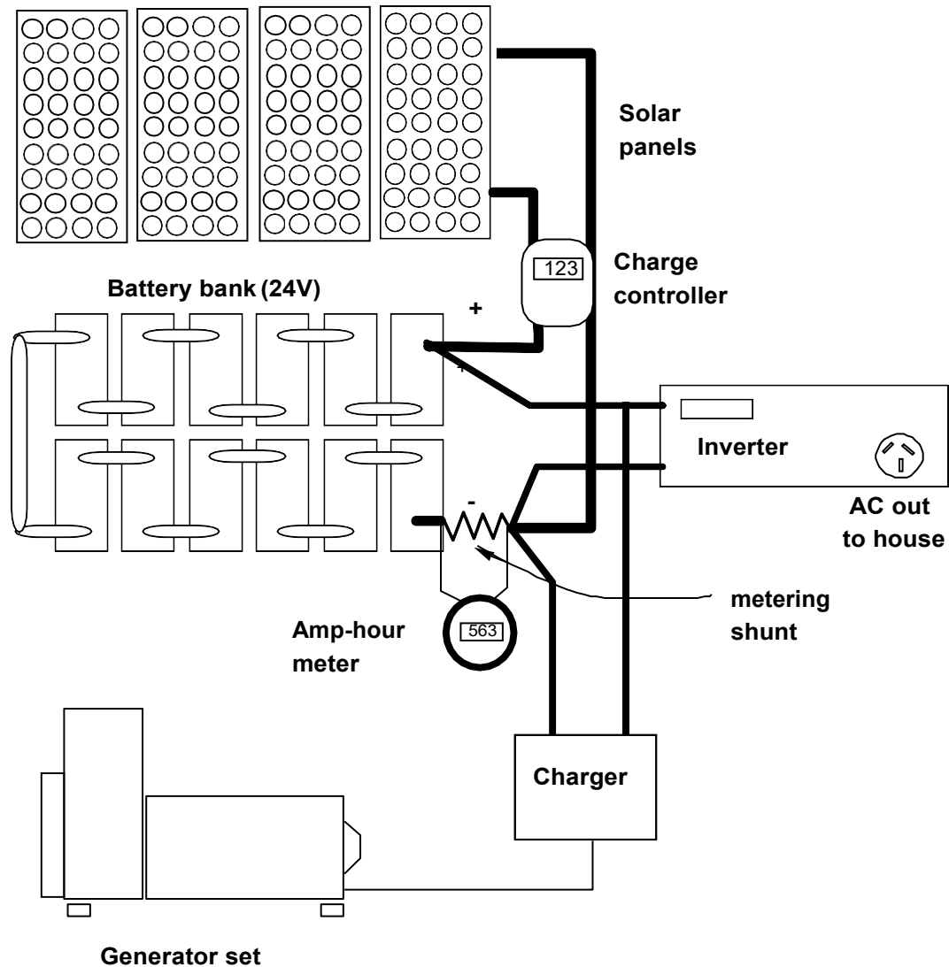
Figure 4 Basic layout of a conventional Photovoltaic Remote Area Power System (RAPS). The solar panels would be normally be mounted as an array, usually on the roof of the building, with the batteries, inverter and charger either within the house or in a purpose built shed. The only unconventional aspect to the design shown here is the Amp Hour meter, which is missing from most systems, and is the subject of some discussion in the text. The generator is usually situated some distance from the house to reduce sound and fumes. You will note that ALL current to and from the battery bank passes through the metering shunt (a very low value resistor, which allows the user to monitor the current entering and leaving the battery bank).
