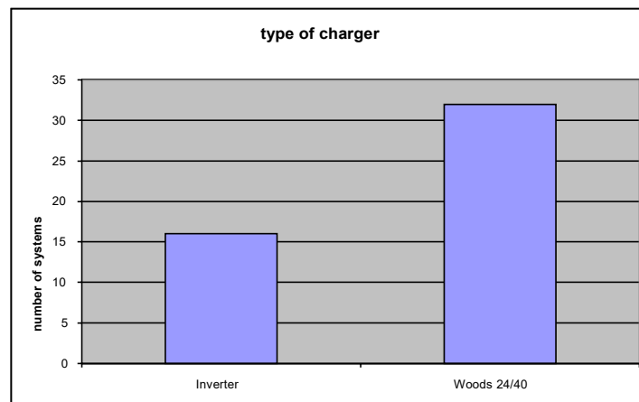
Fig 23 Distribution of charger types. At the time of installation (c 1997) there was a very poor selection of battery chargers available to solar installers - within this sample there are only two options in use – the inverter/charger (which is the most efficient of the charger types) and the Woods charger, which is a conventional full wave linear battery charger with a primitive variable voltage capability. During the course of the survey several households purchased Stanbury stand alone battery chargers, which offer higher currents, and are basically a telco style charger. No household had a stand-alone switchmode charger.
