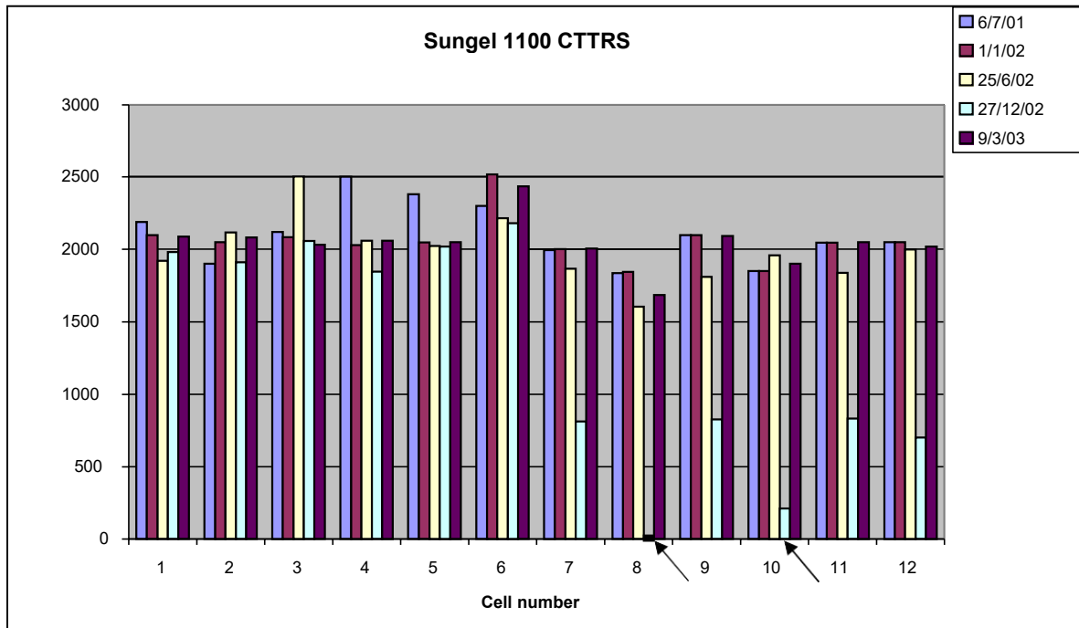
Fig 14. A time series indicating the dramatic effect of the de-sulphator fitted to the only set of GEL cells in the study, those installed at the CTRS power system, Sungel SG1100 (Battery Energy), originally installed in June 2000, replacing the original BP 1100 cells. The de-sulphator was fitted to cells 1-6 on 1 January 02, with cells 7-12 as the control section. Approximately 6 mo later, the conductance of the cells on the test side remained constant or had improved, those on the control side had started to show a decline in conductivity. On the 27 December 02, after a prolonged period of cloudy weather, the system failed, with the conductivity of two cells ( 8 and 10 ) falling to lows of 22 and 209 Siemens ( arrows ) (nominal original value 2000), indicating very severe damage, while the others fell to an average of 700. A second de-sulphator was immediately fitted across cells 7 – 12, and the batteries were brought up to equalisation voltage using the generator and maintained in this state as far as practicable. Conductivity readings on the 9 March 03, indicated that the cells had made good recovery, but cells 8 and 10 had not achieved their pre-collapse conductance levels (and were subsequently replaced). Cells 7 and 9 collapsed in Nov 03. and were replaced. Cells 1-6 have retained their original conductivities.
