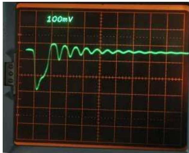
Appendix 1 Fig 3 Oscilloscope trace of the de-sulphator pulse. Scale – 100 mV (1000A) per vertical division (the pulse amplitude is 2500A in this example), 100 nS per horizontal division. The battery resonance is clearly obvious at 17.5 MHz, and the pulse width is 100 nS.
