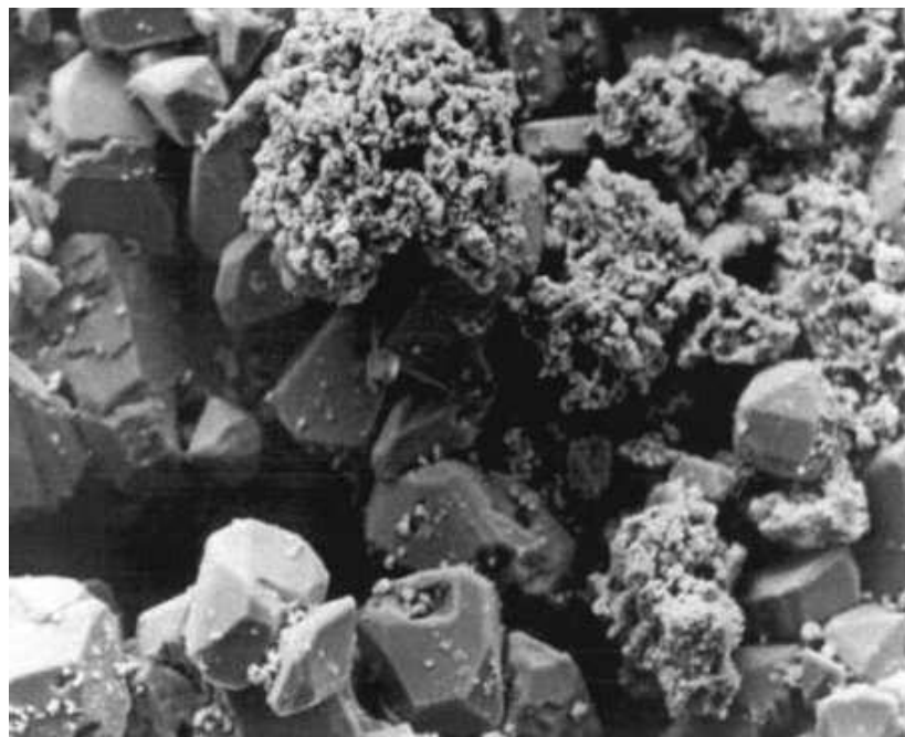
Fig 2 This is an electron microscope picture, magnified 549 times, of a 6 month old battery positive plate used in an ambulance. Given the amount of sulphation, this battery has already reached the end of its service life. Note the large sulphate crystals on the battery plate and the severe erosion of the sponge lead plate material. This battery was never de-sulphated.
