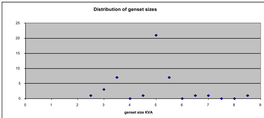
Fig 25 Distribution of Genset capacities. 5KVA 3000 rpm manual start gasoline gensets are the cheapest, most readily available, and have been installed in the majority of systems. They are also extremely noisy and have short lifetimes. Unfortunately because of the limited capabilities of the battery chargers (1.2 kW at the most – due to design constraints that prevent “linear” chargers from utilising more than 40% of the genset capacity) the capacity of these gensets is rarely used, and result in substantial fuel inefficiencies (unless the householder uses the excess load to perform tasks requiring higher power (drying, vacuuming)).
