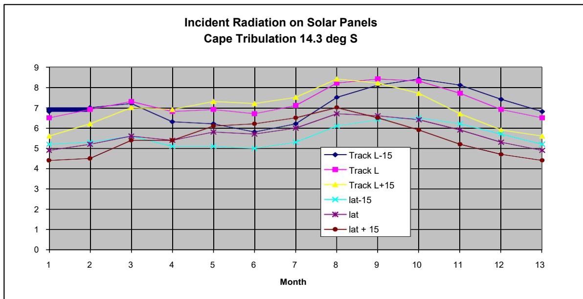
Fig 27 Effect of PV array angle versus month on incident solar radiation at Cape Tribulation, for both fixed arrays and single-axis trackers with the panel array facing true north. The effects of incorrect array angle on received solar power can be quite dramatic. The three lower traces are for fixed arrays, the top three traces are for a single-axis tracker (which also require seasonal adjustment). The angle of the array is commonly specified as the same angle as the latitude of the site, plus or minus 15 degrees, depending on the season. Cape Tribulation is 14.3 degrees south, and the 3 angles would be 0.5 deg (lat-15), 14.3 (lat), and 29.3 deg. (lat+15) for summer, mid season and winter respectively. Y axis = KWH/ m 2 /day falling on the solar collector. X axis – month (Month 13 = Jan for graphical completeness) The solar constant - the amount of solar energy received on 1 square meter of horizontal surface - is approximately 1 KW/ m 2 (remember that the collector only yeilds 15 to 18 percent of this figure as electric power). (data produced with “Solar Sizer” - Solar Energy International, Carbondale Co. USA.)
