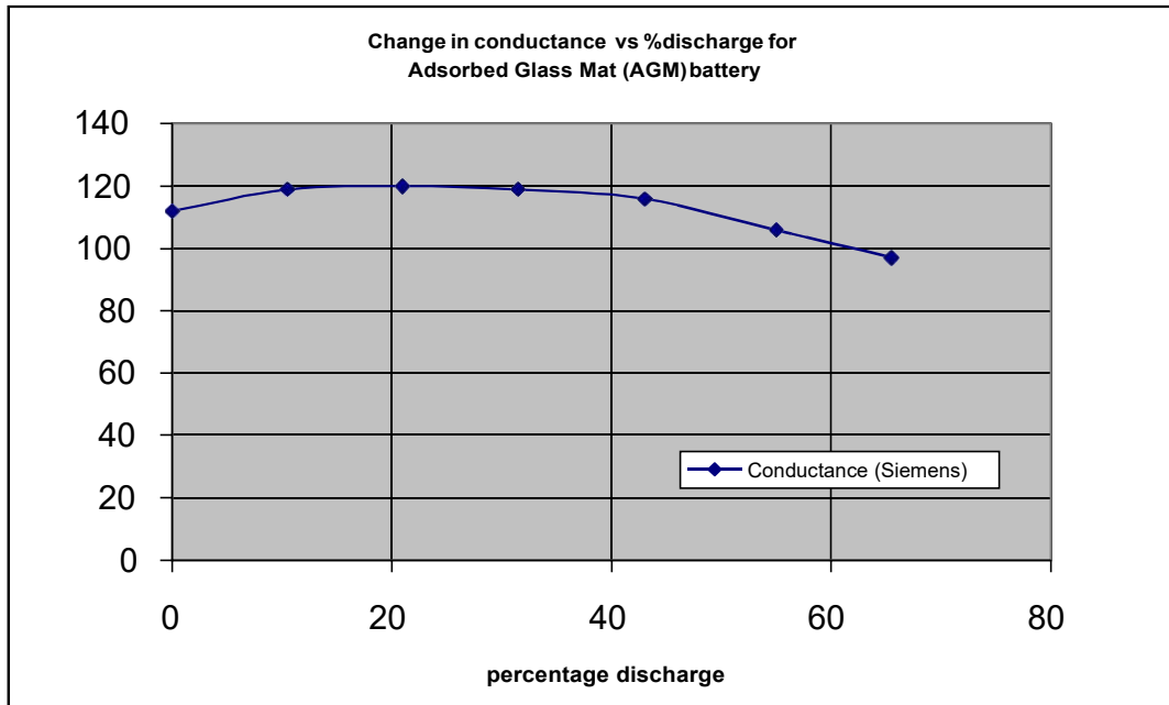
Fig 9 Change in conductance (in Siemens, vertical axis) as a function of the discharged state of the battery - in this case an old 12V Hawker AGM battery with a nominal starting conductance of 120 Siemens (26AH). It is evident that the conductance only significantly reduces when the battery discharge level reaches about 60%. As a result, the conductance readings give a fairly good approximation as to battery “State of Health” – at least for relatively well charged cells.
