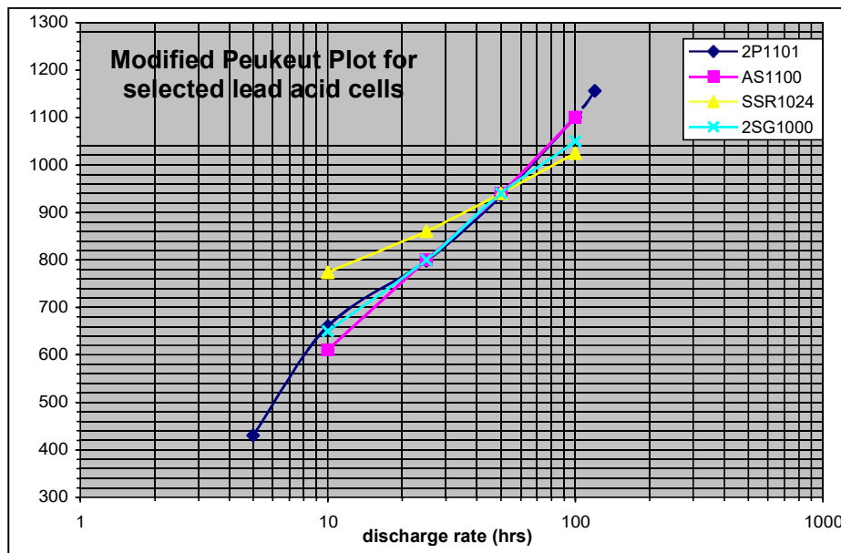
Fig 29 Peukeut plot of cell capacity (in ampere-hours) vs discharge rate (discharge of the total rated capacity over a designated time) of 4 battery types all having comparable published capacities, and which are representative of the battery types used in the Daintree area. Rather than plotting these curves as a log-log plot, the Y axis has been plotted on a linear scale to visually enhance the differences between the cell types. It can be seen that as the discharge rate increases (moving to the left on the X axis) the rated capacity falls sharply.
